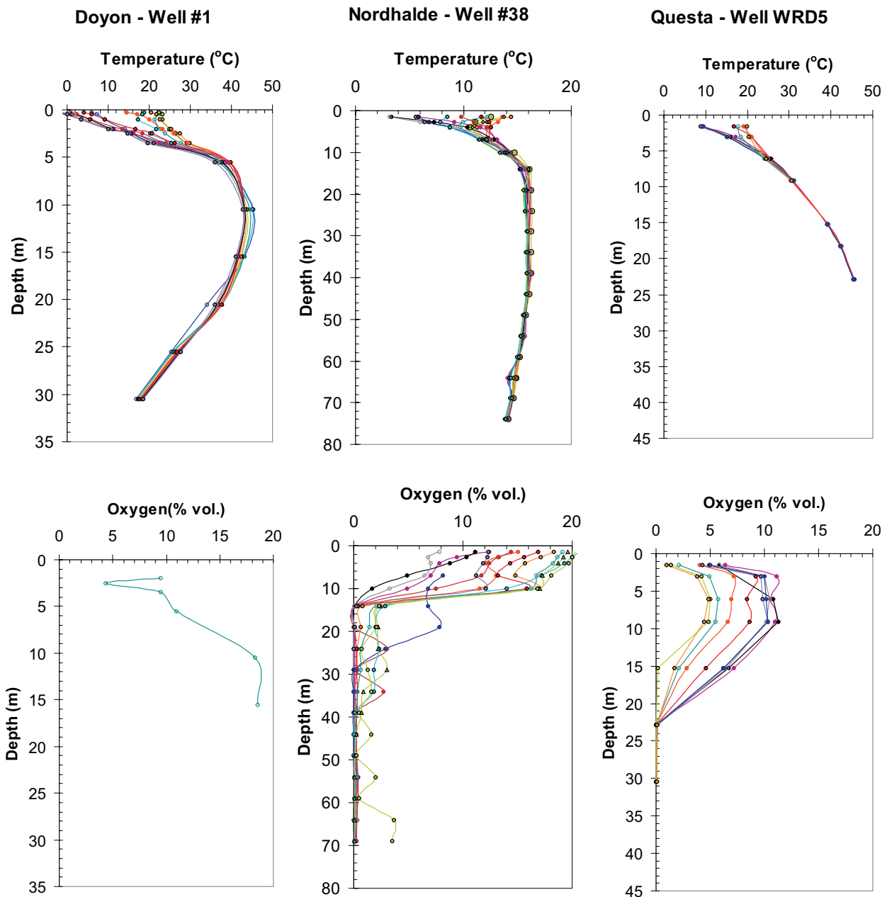
FIG 5 - Temperature and oxygen profiles in three waste rock piles: Doyon Mine in Canada, Nordhalde in Germany and Questa in the USA.
