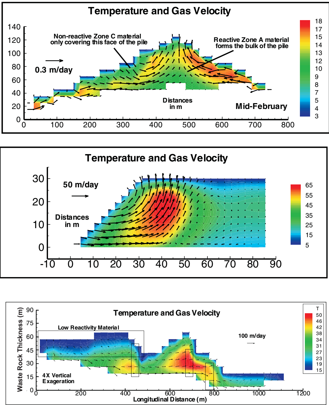
FIG 6 - Simulated temperature and gas velocity for the Nordhalde (top, Lefebvre et al , 1998), Doyon (centre, Lefebvre, 1994) and Questa (bottom, Lefebvre et al , 2002) waste rock piles.
