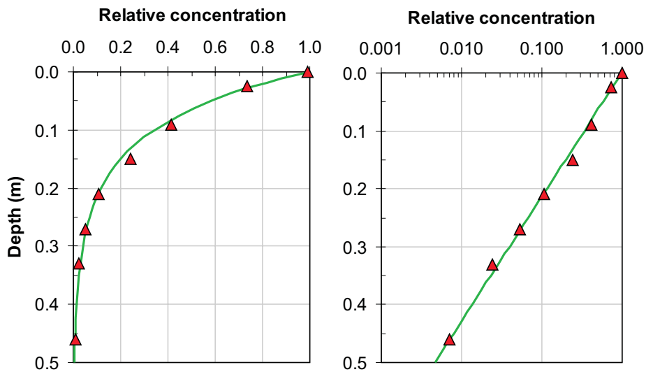
FIG 1 - Relative oxygen concentration in a mine tailings column (after Yanful, 1991).
