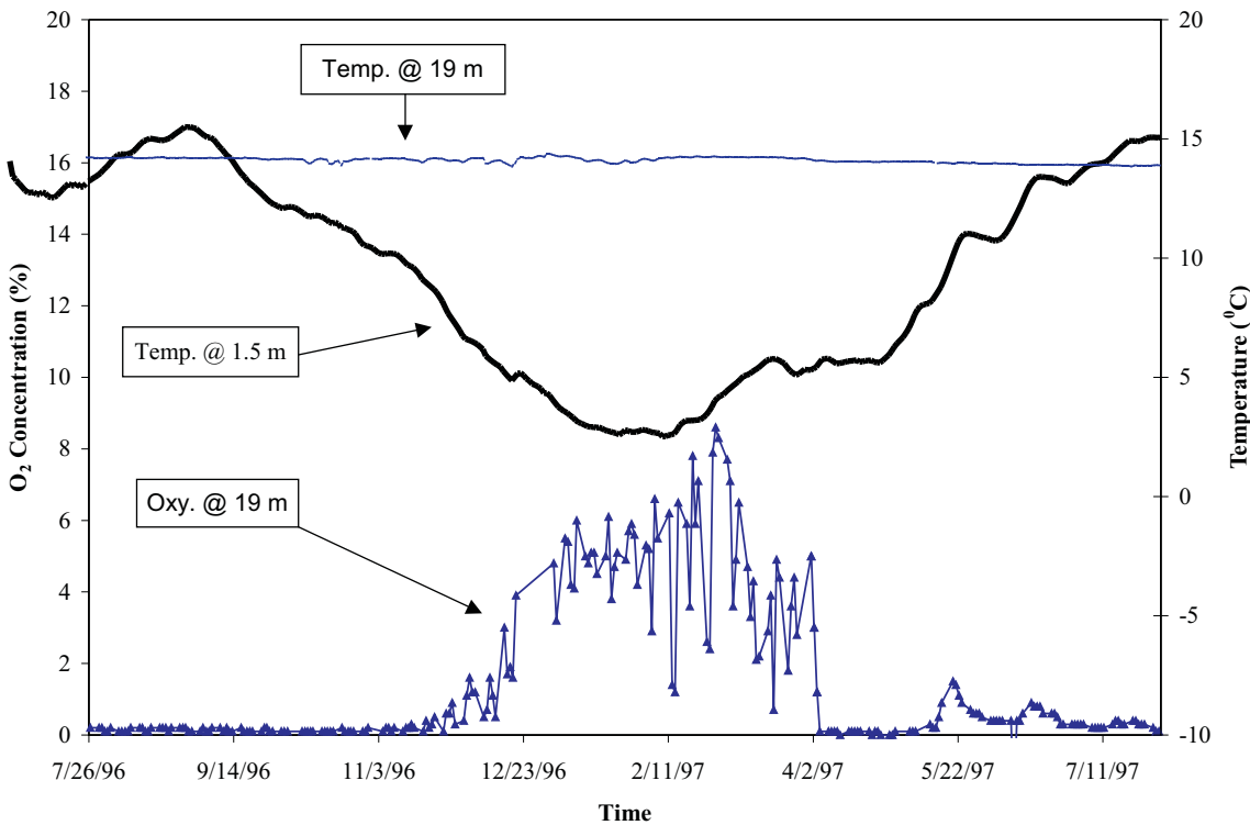
FIG 3 - Relationship of oxygen concentrations in the 19 m port to temperatures in the 1.5 m and 19 m ports for Borehole 36, Nordhalde, Germany (from Smolensky et al , 1999).
