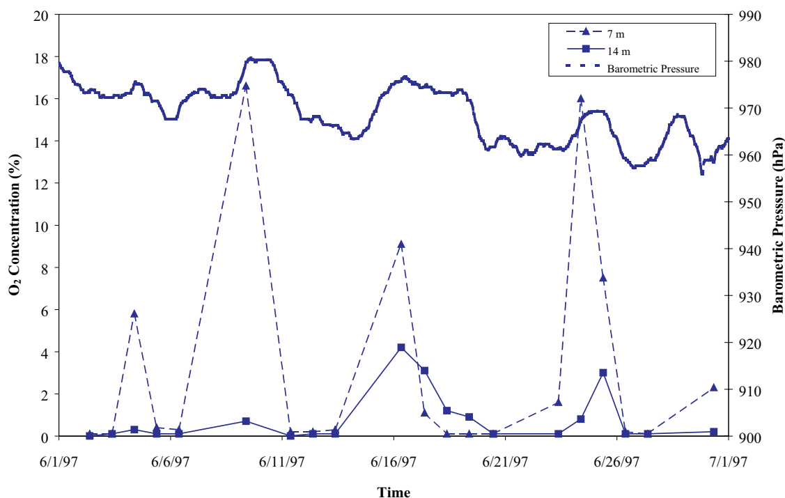
FIG 4 - Fluctuations in oxygen concentrations and barometric pressure for Borehole 37, Nordhalde, Germany (from Smolensky et al , 1999).
