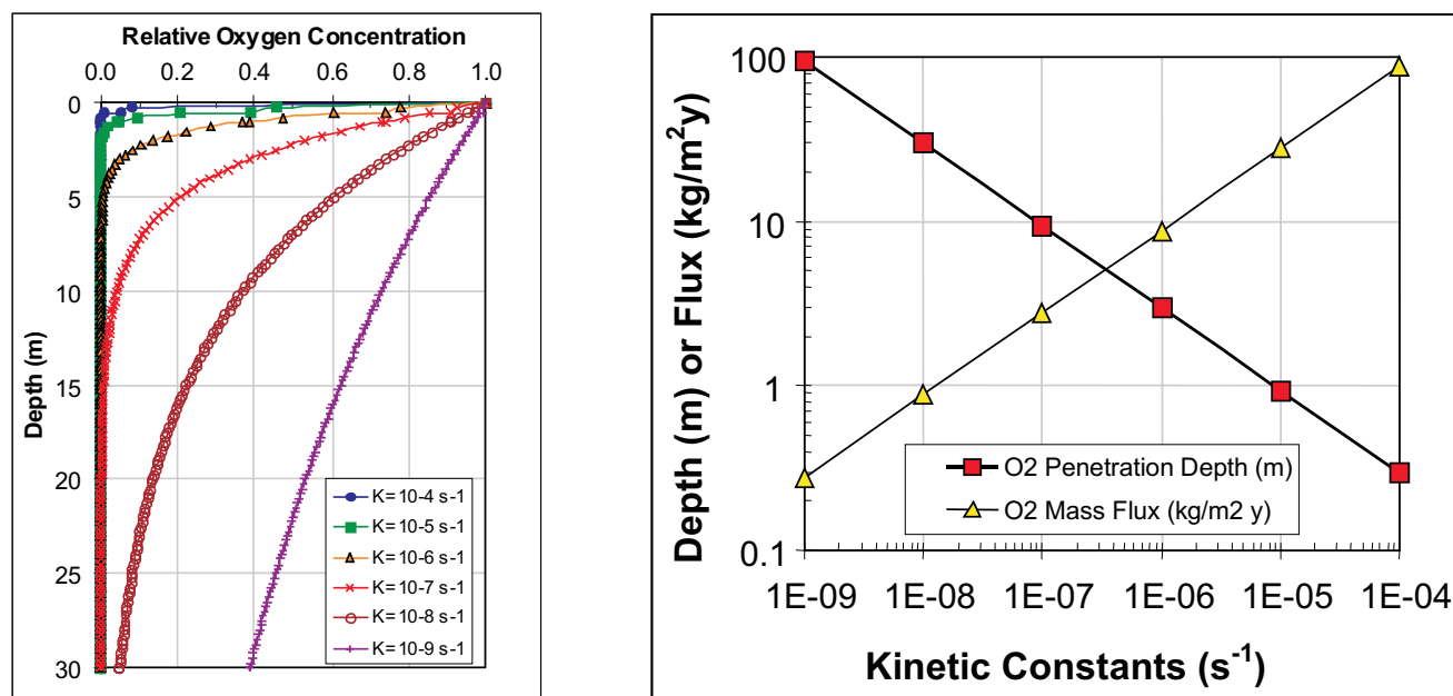
FIG 2 - Oxygen diffusion as a function of the oxidation kinetics constant K ( s^{-1} ). Left: oxygen profiles versus depth. Right: oxygen penetration depth at which the relative concentration is 0.05 and the related oxygen mass flux from the surface.
